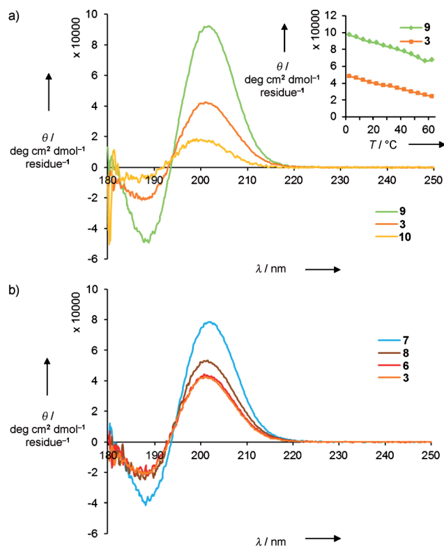
Figure 1. Circular dichroism spectra of oligoureas with pyrrolidine junction in TFE. a) Spectra for the 4-mer 10 and 7-mers 3 and 9 . Inset: temperature dependence of the CD signal of 3 and 9 at \lambda = 203 nm between 0°C and 60°C in TFE. b) Spectra for the 7-mer 3 , 11-mer 6 , 15-mer 8 , and 20-mer 7 . Samples were studied at 0.1 or 0.2 mm.
