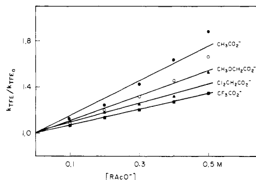
Figure 1. General base catalysis by carboxylate anions of the reaction between trifluoroethanol and the 1-(4-methoxyphenyl)ethyl cation in 50:45:5 (v/v/v) \text{H}_2\text{O}:\text{TfE}:\text{MeOH} at ionic strength 0.5 maintained with \text{NaClO}_4 . The y axis gives the normalized yield of the trifluoroethyl ether calculated from the trifluoroethyl ether:azide adduct product ratio as described in the text.
