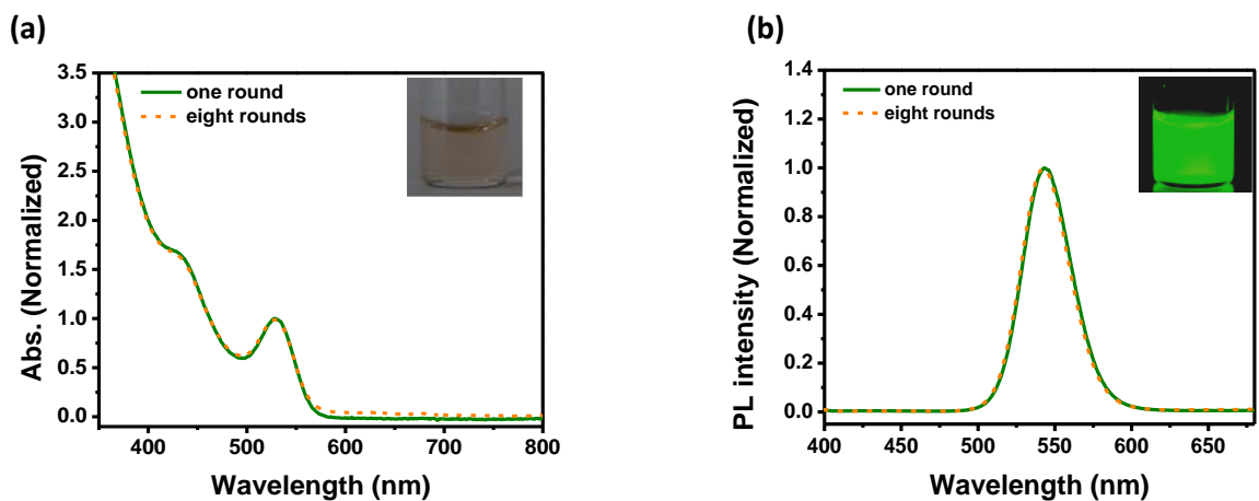
Figure 5. (a) UV-vis absorption (b) and PL spectra of dispersions of bis(LA)-PEG-OCH 3 -QDs ( \lambda_{em} =540 nm) after one (green) and eight rounds (orange) of purification using a centrifugal membrane device as described in the text. The absorption and PL spectra were normalized with respect to the band edge peak and the emission maximum, respectively. The insets show the white light and fluorescence images of the bis(LA)-PEG-OCH 3 -QDs after eight rounds of purification then dispersed in DI water.
