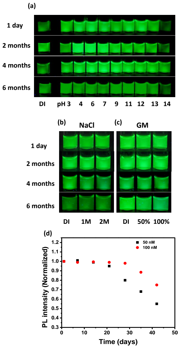
Figure 3. (a-c) Fluorescence images of dispersions of QDs ( \lambda_{em} = 540 nm) photoligated with bis(LA)-PEG-OCH 3 (at 0.5 \mu M): (a) in 10 mM PBS buffer at different pH values from 3 to 14; (b) in the presence of 1 and 2 M NaCl; (c) in the presence of 50% and 100% RPMI growth media (GM). (d) Plot of PL intensity versus storage time of QDs ( \lambda_{em} =540 nm) photoligated with bis(LA)-PEG-OCH 3 at different concentrations of 50 nM and 100 nM. The samples were stored at ambient conditions with exposure to room light.
