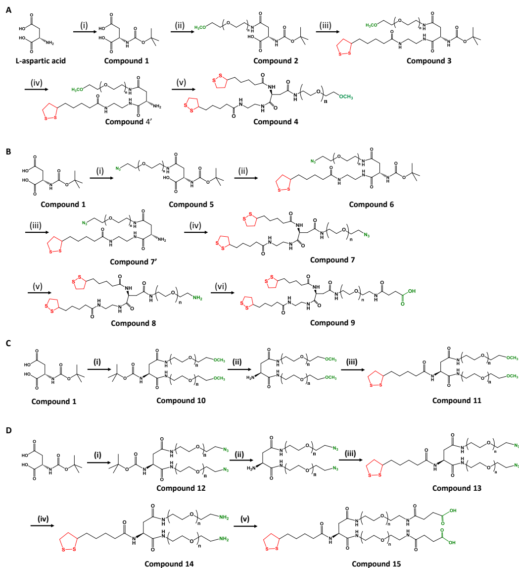
Figure 1. Schematic representation of the chemical structures and synthetic steps used to prepare the various ligands including: (A) bis(LA)PEG-OCH 3 , (i) Boc 2 O (di-tert-butyl dicarbonate); (ii) NH 2 -PEG-OCH 3 , DCC (N,N'-dicyclohexylcarbodiimide); (iii) LA-ethylenediamine, DCC, HOBT·H 2 O (hydroxybenzotriazole monohydrate); (iv) 4 M HCl in dioxane; (v) LA (lipoic acid), DCC, DMAP (4-dimethylaminopyridine); Only one isomer in step (ii) is shown (as a representative compound); (B) bis(LA)-PEG-N 3 /NH 2 /COOH, (i) NH 2 -PEG-N 3 , DCC; (ii) LA-ethylenediamine, DCC, HOBT·H 2 O; (iii) 4 M HCl in dioxane; (iv) LA (lipoic acid), DCC, DMAP; (v) PPh 3 (triphenylphosphine), H 2 O; (vi) succinic anhydride, Et 3 N; (C) LA-(PEG-OCH 3 ) 2 , (i) NH 2 -PEG-OCH 3 , DCC, HOBT·H 2 O; (ii) 4 M HCl in dioxane; (iii) LA (lipoic acid), DCC, HOBT·H 2 O; (D) LA-(PEG-N 3 /NH 2 /COOH) 2 , (i) NH 2 -PEG-N 3 , DCC, HOBT·H 2 O; (ii) 4 M HCl in dioxane; (iii) LA (lipoic acid), DCC, HOBT·H 2 O; (iv) PPh 3 , H 2 O; (v) succinic anhydride, Et 3 N.
