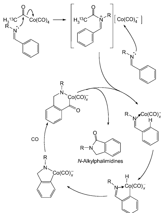
Scheme 4. Proposed Mechanism for the Formation of N-Alkylphthalimidines from Benzaldimines and CO in the Presence of [\text{Co}(^{13}\text{CH}_3\text{C}(\text{O}))(\text{CO})_3(\text{P}(\text{o-tol})_3)]^1
