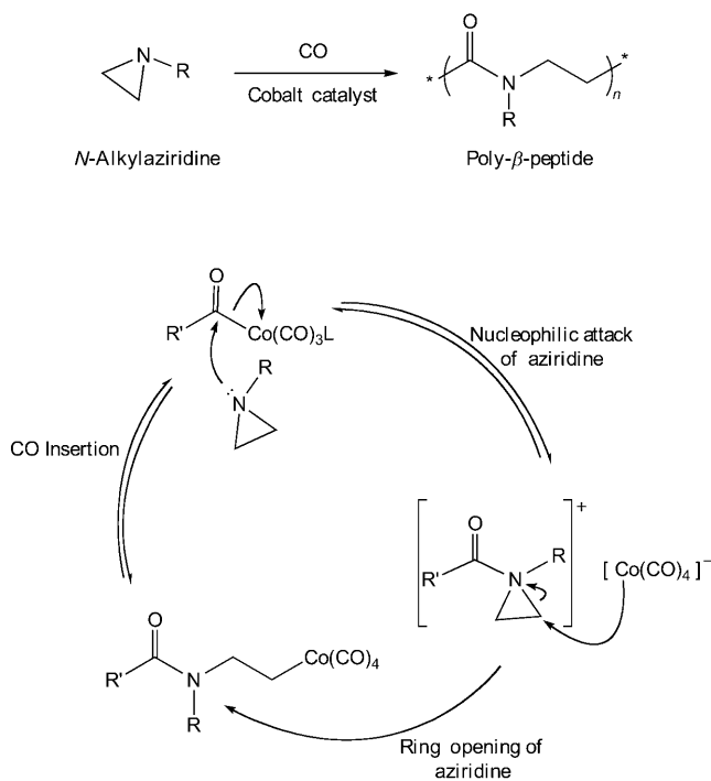
Scheme 3. Copolymerization of N -Alkylaziridines with CO to Form Poly- \beta -peptides, and Proposed Mechanism
