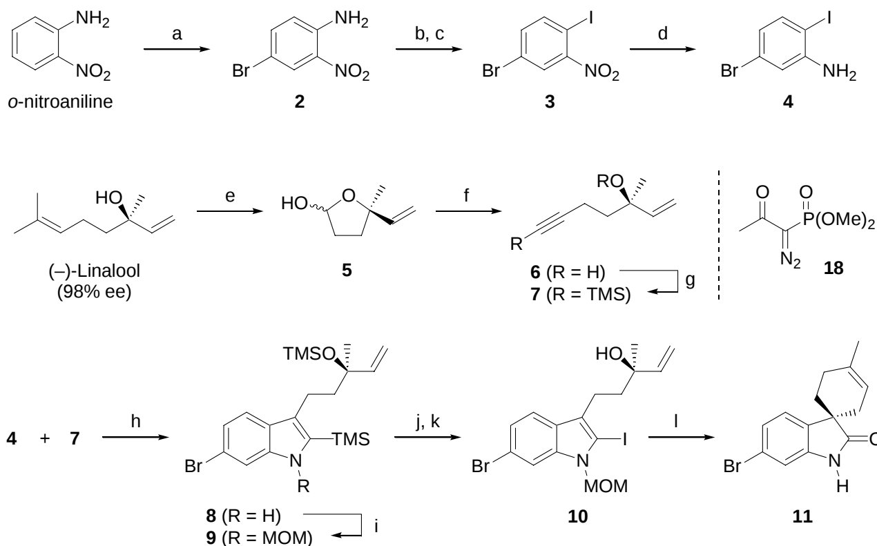
Scheme 3. Reagents and conditions: (a) aq. HBr, aq. H 2 O 2 , MeOH, 0 °C→rt, 75%; (b) BF 3 ·OEt 2 , t -BuONO, THF, −30 °C; (c) KI, I 2 , rt, 88% (2 steps); (d) Fe, AcOH-EtOH, reflux, 91%; (e) O 3 , then Me 2 S, CH 2 Cl 2 -pyridine, −78 °C, 66%; (f) 18 , K 2 CO 3 , MeOH, rt, 71%; (g) n -BuLi, THF, −78 °C, then TMSCl, −78 °C→rt, 92%; (h) Pd(OAc) 2 , PPh 3 , LiCl, K 2 CO 3 , DMF, 100 °C, 57%; (i) NaH, MOMCl, THF-DMF, 0 °C, 97%; (j) NIS, CH 2 Cl 2 , reflux; (k) TBAF, THF, 0 °C, 94% (2 steps); (l) CuCl, 2-aminopyridine, NaOMe-MeOH, triglyme, 100 °C, 69%.
