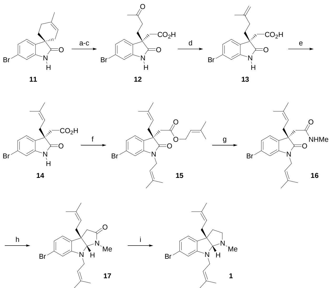
Scheme 5. Reagents and conditions: (a) OsO 4 , NMO, acetone-H 2 O, rt; (b) NaIO 4 , THF-H 2 O, rt; (c) NaClO 2 , NaH 2 PO 4 ·2H 2 O, 2-methyl-2-butene, t -BuOH-H 2 O-THF, rt, 84% (3 steps); (d) Ph 3 PCH 3 Br, n -BuLi, THF, -25 °C→rt; (e) H 2 SO 4 , then MgSO 4 , 1,4-dioxane, 60 °C; (f) prenyl bromide, K 2 CO 3 , acetone, reflux, 18% (for 3 steps); (g) aq. MeNH 2 , MeOH, rt, 67%; (h) AlH 3 ·EtNMe 2 , THF, -20 °C, 96%; (i) AlH 3 ·EtNMe 2 , THF, rt, 93%.
