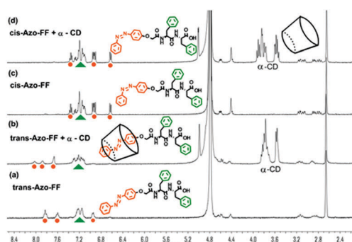
Fig. 1 Partial ^1\text{H} NMR spectra (400 MHz, \text{D}_2\text{O}:\text{DMSO}-d_6(v/v) 9 : 1, 25 ^\circ\text{C} ) of (a) trans -Azo-FF, (b) trans -Azo-FF + \alpha -cyclodextrin (1 : 1), and (c) after 365 nm irradiation of (a) and (d) after 365 nm irradiation of (b), Azo-FF = [ \alpha -cyclodextrin] = 1 mM.
