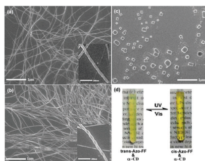
Fig. 3 SEM images of (a) nanofibers formed by trans -Azo-FF and (b) nanohelices formed by trans -Azo-FF/ \alpha -cyclodextrin. (c) trans -Azo-FF/ \alpha -cyclodextrin after being irradiated by UV light (365 nm) for 3 min. (d) Photograph of Azo-FF/ \alpha -cyclodextrin solution under UV and visible light.
