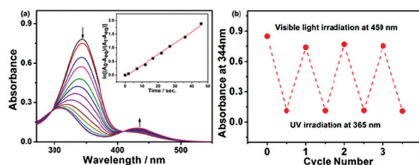
Fig. 2 (a) UV-vis spectra of Azo-FF/ \alpha -cyclodextrin (1 : 1) (0.03 mM in \text{H}_2\text{O} ) to determine the photoisomerization rate constant ( k_t ) in water. The duration of UV light was set at 0 \rightarrow 121 s at 365 nm. Inset: Determination of the k_t value of Azo-FF/ \alpha -cyclodextrin (1 : 1) upon exposure to UV light at 365 nm. (b) Cyclic responses of the absorbance values at 344 nm of trans -Azo-FF/ \alpha -cyclodextrin solution (0.03 mM) on alternating irradiation between UV and visible light.
