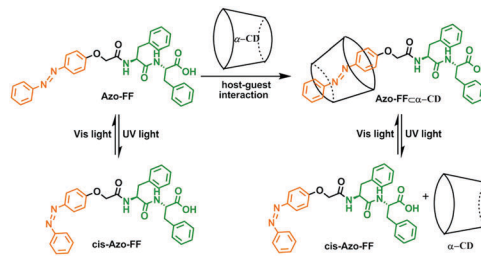
Scheme 2 Self-assembly/disassembly based on the photo-responsive interconversion of Azo-FF and \alpha -cyclodextrin.
