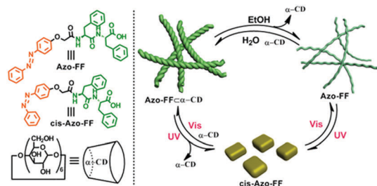
Scheme 1 Structural illustration of the host and guest and the dual-controlled conversion of self-assembly.
