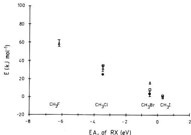
Figure 5. Activation energy E for the reactions \text{Me} + \text{RX} \rightarrow \text{MeX} + \text{R} (given in Table 6) as a function of the vertical electron affinity \text{EA}_v of RX (□ Cu; Δ K; ● Cu with E obtained using the three-parameter expression).
