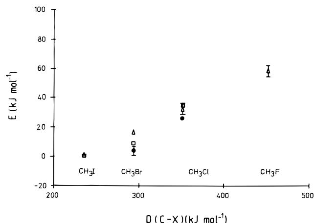
Figure 6. Activation energy E for the reactions \text{Me} + \text{RX} \rightarrow \text{MeX} + \text{R} (given in Table 6) as a function of the dissociation energy of the C–X bond in RX (□ Cu; Δ K; ● Cu with E obtained using the three-parameter expression).
