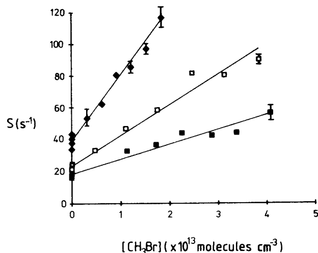
Figure 2. Absolute value S of the slope of eq 5 as a function of CH 3 Br concentration for three different temperatures: (■) 390 K, (□) 516 K, (◆) 702 K.
