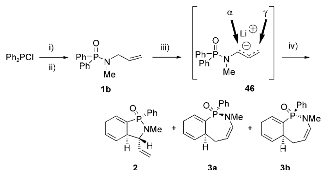
Scheme 6. Synthesis of N -allylphosphinamide 1b and subsequent dearomatization reaction: i) \text{MeNHCH}_2\text{CH}=\text{CH}_2 , \text{NEt}_3 (2.5 equiv), toluene, -78^\circ\text{C} ; ii) \text{H}_2\text{O}_2 (1 equiv), -30^\circ\text{C} , THF; iii) RLi (2.5 equiv), DMPU (6 equiv), THF, -90^\circ\text{C} , t_1 ; iv) 2,6-di- tert -butyl-4-methylphenol (5 equiv), -90^\circ\text{C} , 30 min.
