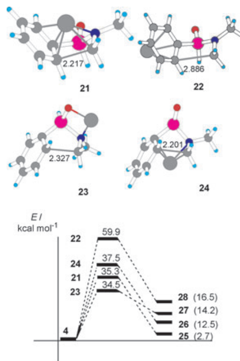
Figure 7. Transition structures, activation barriers and reaction energies for the cyclisation reaction of anion 4 . Bond lengths in Å. For the colour code see the legend of Figure 3.
