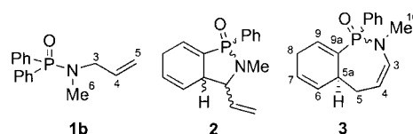
Figure 1. N -Allylphosphinamide 1b and five- and seven-membered ring cyclisation products 2 and 3 .
