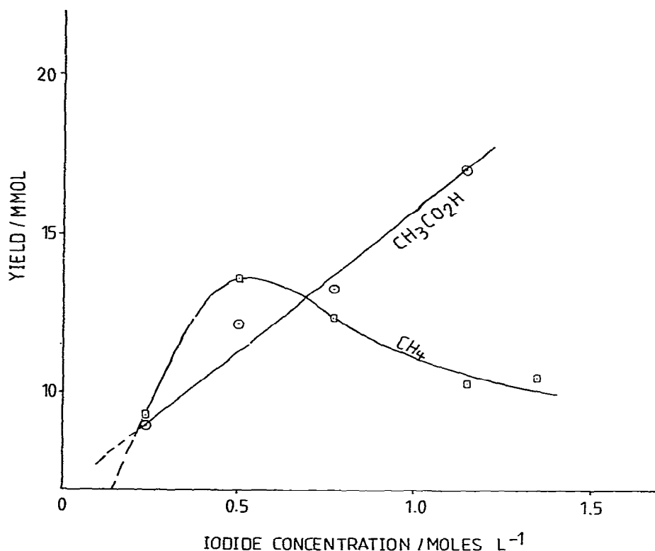
Fig. 2. Effect of iodide concentration on yields of \text{CH}_3\text{CO}_2\text{H} and \text{CH}_4 . \text{H}_2 partial pressure 5.1 bar. Other conditions as for Fig. 1, but with amount of HI varied.
