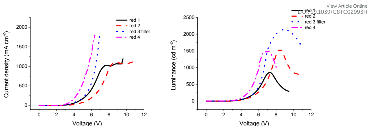
Figure 3: Current density and luminance vs voltage for compounds 1 – 4 .
