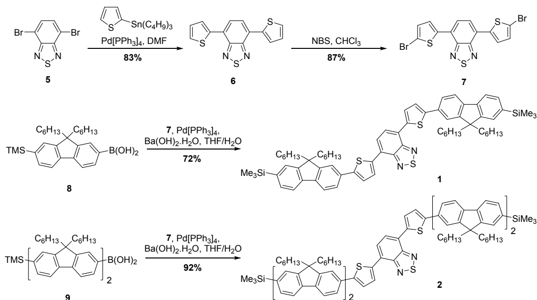
Scheme 1: Synthesis of compounds 1 and 2 .
