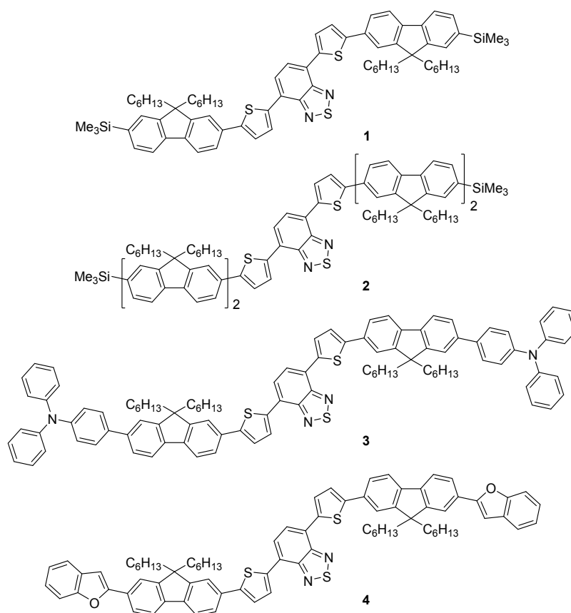
Figure 1: Structures of the molecular emissive species, compounds 1–4 .
