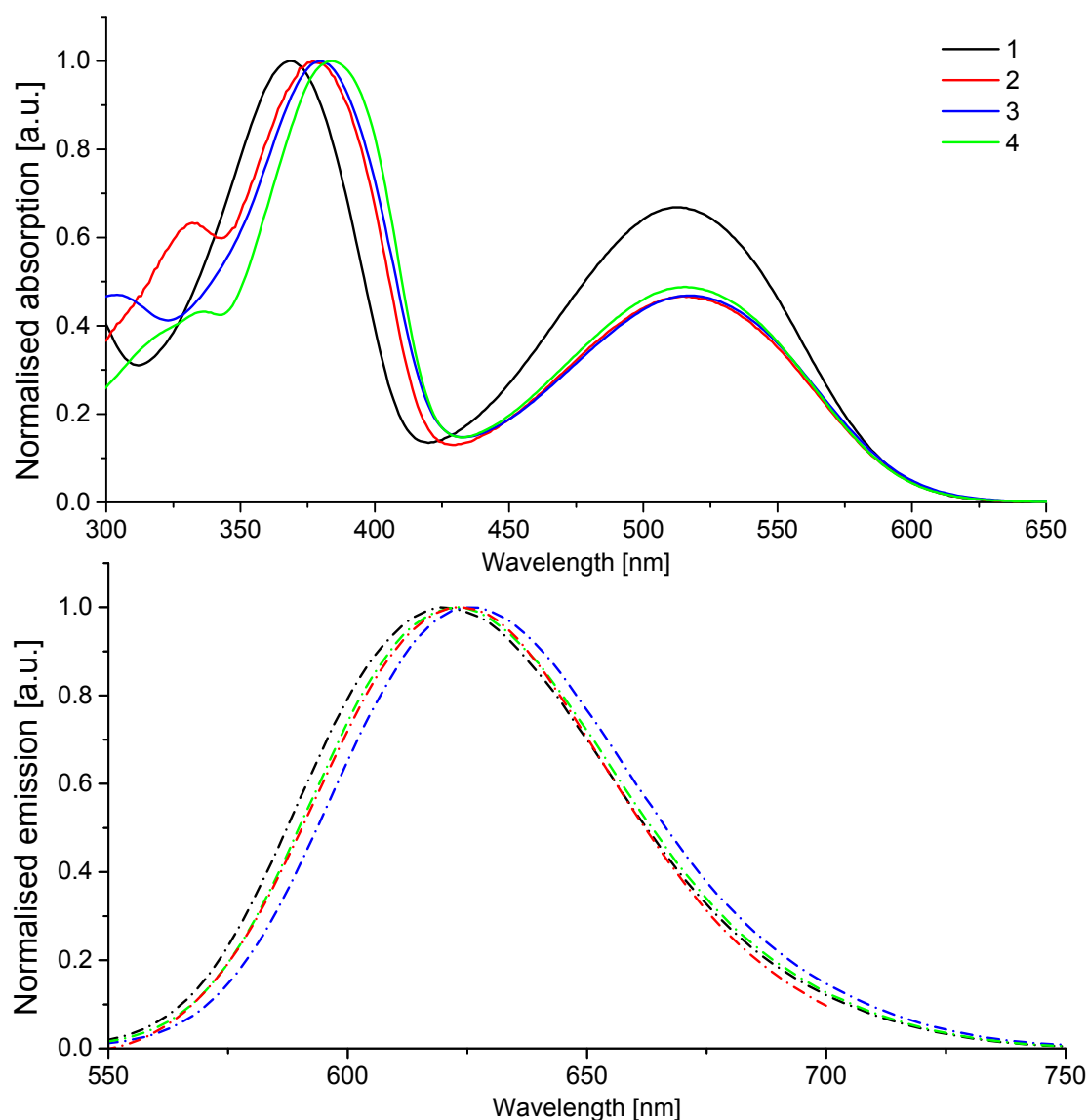
Figure 2: Absorption (top) and emission (bottom) in dichloromethane solution for compounds 1-4 .
