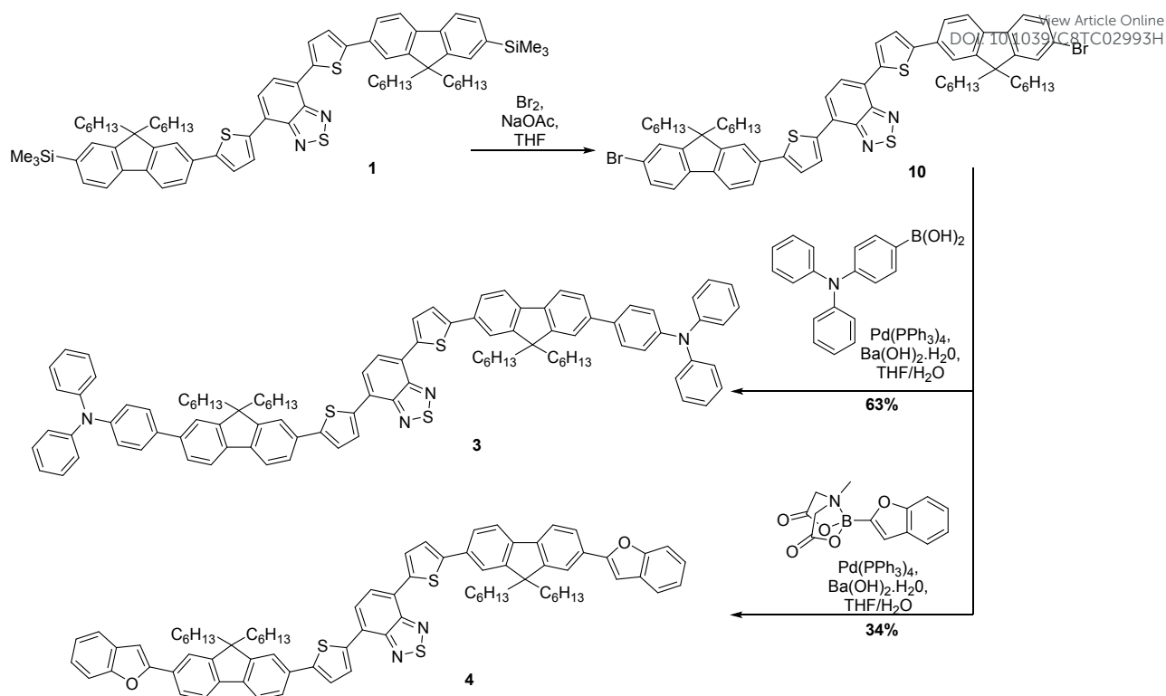
Scheme 2: Synthesis of compounds 3 and 4 . Note that compound 10 was isolated as a mixture.
