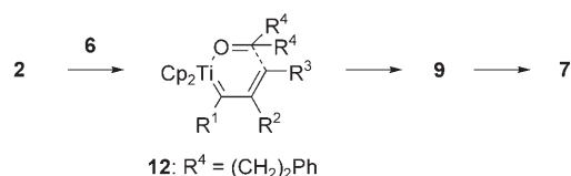
Scheme 5. A possible pathway for the formation of homoallyl alcohols 7 by the reaction of vinyl carbene complexes 2 with 6 .
