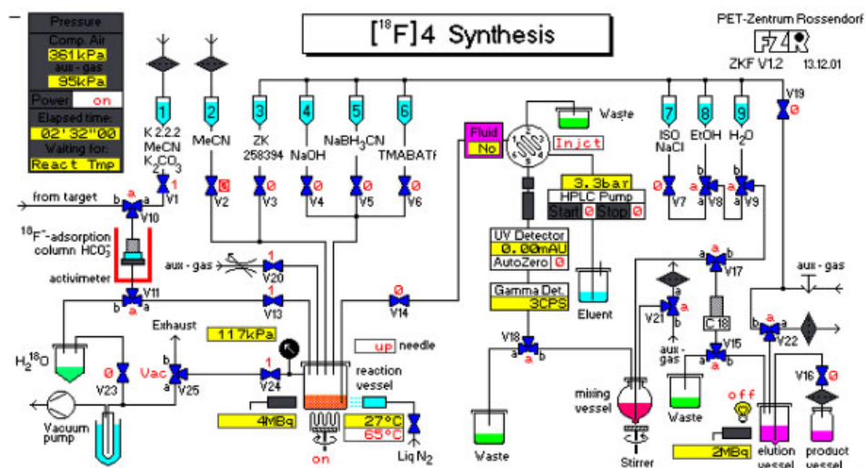
Figure 1. Schematic diagram of the module for synthesizing [^{18}\text{F}]\mathbf{4}
