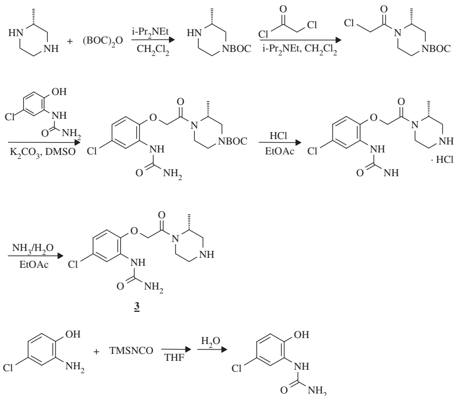
Scheme 3. Synthesis of the piperazine derivative 3
