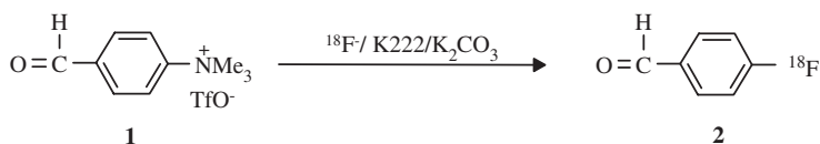
Scheme 2. Synthesis of 4-[ ^{18}\text{F} ]fluorobenzaldehyde ( 2 )
