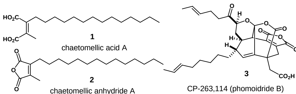
Figure 1. Natural farnesyltransferase inhibitors.
