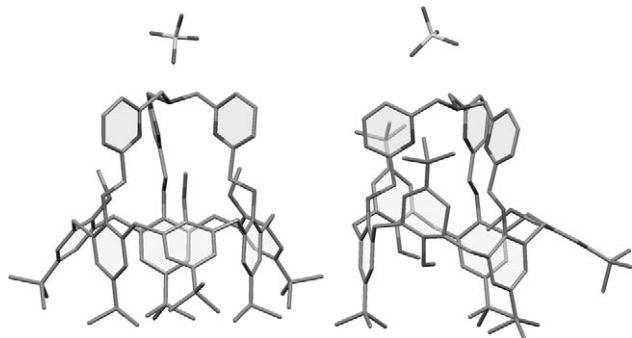
Figure 3. Crystal structure of 11 ·H + ·ClO 4 − . Left: one of the two cone conformations (see the text); Right: 1,3-alternate conformation. Hydrogen atoms and some crystallization solvent molecules have been omitted for clarity.
