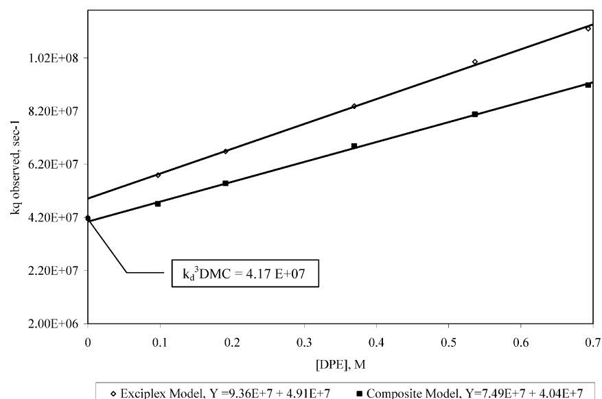
Figure 10. Quenching curves generated by the first-order sequential two reaction model and by the composite 3 DPE and head-to-tail 3 biradical model.
