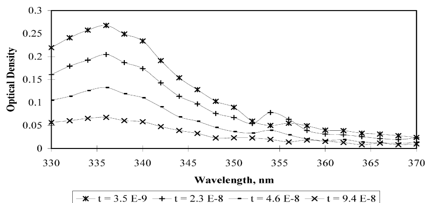
Figure 5. Time-resolved absorption spectrum for the DMC-DPE temporal signal, \lambda_{\text{max}} = 337 nm.
