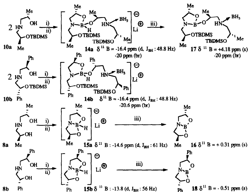
Scheme 5 : Preparation of chiral aminoborohydrides.
