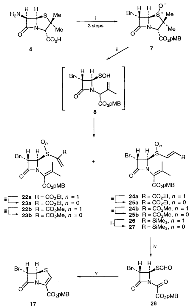
Scheme 3 Reagents and conditions: i, See (i), (ii) and (iii) in Scheme 2; ii, (a) \text{HC}\equiv\text{CR} , toluene, reflux, 3 h; (b) \text{Et}_3\text{N} (0.1 mol equiv.), \text{CH}_2\text{Cl}_2 , 25 °C; iii, \text{PBr}_3 , DMF, –10 °C, 20 min; iv, (a) \text{O}_3 , \text{EtOAc} , –76 °C; (b) aq. \text{Na}_2\text{SO}_3 – \text{Na}_2\text{S}_2\text{O}_5 (pH 7.0); v, \text{P(OMe)}_3 (5 mol equiv.), toluene, 50 °C, 1 h
