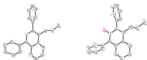
Figure 1. ORTEP drawings of 3ag and 5ag .
