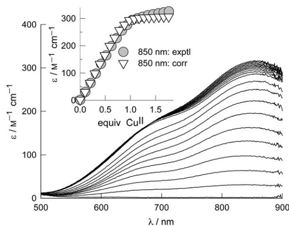
Figure 5. Visible spectra taken over the course of the titration of a solution of 4 ( 2.075 \times 10^{-3}\text{M} ) in DMSO against \text{Cu}^{\text{II}}(\text{CF}_3\text{SO}_3)_2 . The two bands at 750 and 850 nm indicate the formation of a trigonal-bipyramidal complex. Inset are titration profiles of the band at 850 nm: experimental values (●); values corrected for the absorbance of the [\text{Cu}^{\text{II}}(\text{dmsO})_4]^{2+} species (▼).
