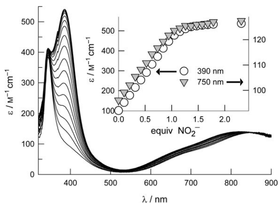
Figure 4. Visible spectra taken over the course of the titration of a solution of [\text{Cu}^{\text{II}}(\text{2})](\text{ClO}_4)_2 ( 3.74 \times 10^{-3}\text{M} ) in DMSO against [\text{Bu}_4\text{N}]\text{NO}_2 . Inset: titration profiles at selected wavelengths.
