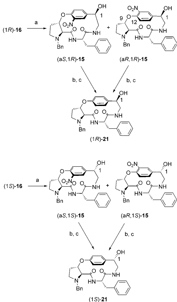
Scheme 6. S N Ar-based cycloetherification of (1 R )- 16 and (1 S )- 16 . a) TBAF, DMSO, powdered 4 Å molecular sieves, 60 °C, 70% yield, atropenantioselectivity of (a S ,1 R )- 15 /(a R ,1 R )- 15 = 1:1.6 and of (a S ,1 S )- 15 /(a R ,1 S )- 15 = 1:1.4; b) H 2 , Pd/C, MeOH/EtOAc (1:1); c) NaNO 2 , H 3 PO 2 , Cu 2 O (0.1 equiv), SnCl 2 (0.2 equiv). TBAF = tetrabutylammonium fluoride, DMSO = dimethylsulfoxide.
