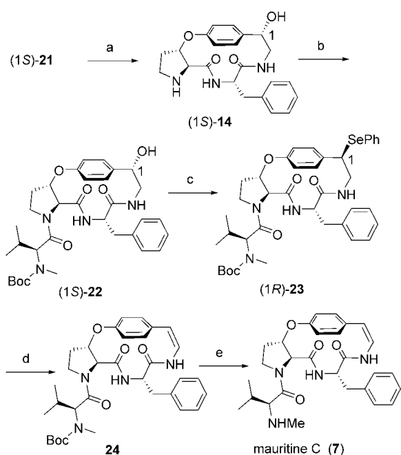
Scheme 7. Synthesis of mauritine C ( 7 ). a) \text{H}_2 , Pd/C, MeOH, 82%; b) N -Boc- N -methyl-L-valine, HATU, DIEA, DMF, 87%; c) 1. MsCl, \text{Et}_3\text{N} , \text{CH}_2\text{Cl}_2 , 2. (\text{PhSe})_2 , \text{NaBH}_4 , EtOH, 74%; d) 1. \text{H}_2\text{O}_2 , pyridine, \text{CH}_2\text{Cl}_2 , 2. benzene, 60°C, 48%; e) TFA, \text{CH}_2\text{Cl}_2 , 78%. HATU = N -[(dimethylamino)-1 H -1,2,3-triazole[4,5- b ]-pyridin-1-ylmethylene]- N -methylmethanaminium hexafluorophosphate, DIEA = N,N -diisopropylethylamine, Ms = mesyl = methanesulfonyl, TFA = trifluoroacetic acid.
