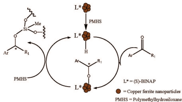
SCHEME 2. Possible Mechanism of Asymmetric Hydrosilylation Catalyzed by Copper Ferrite Nanoparticles
