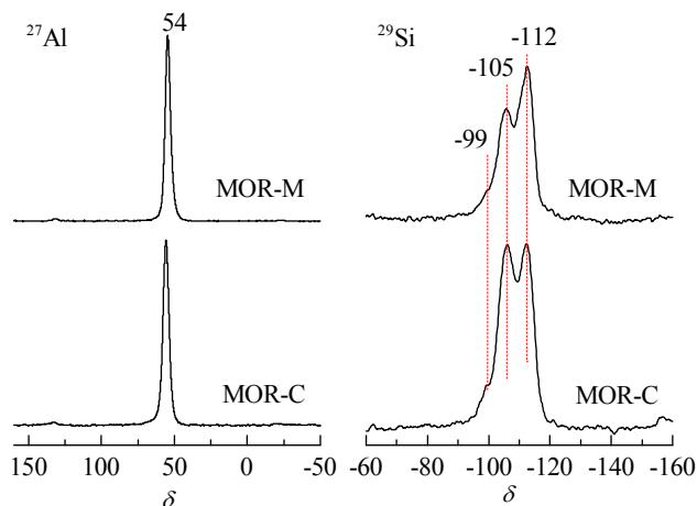
Fig. 4. 27 Al and 29 Si MAS NMR spectra of MOR-M and MOR-C.
