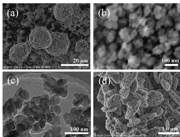
Fig. 2. (a) Low-magnification SEM micrograph of MOR-M; (b) High-magnification SEM micrograph of MOR-M; (c) TEM micrograph of MOR-M; (d) SEM micrograph of MOR-C.
