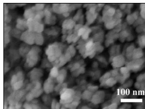
Nanocrystal-assembled MOR
