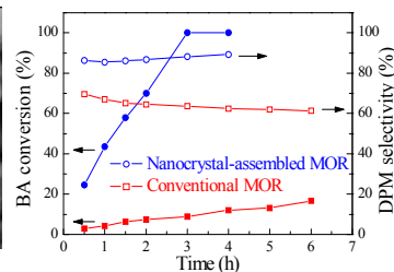
Nanocrystal-assembled MOR
