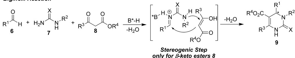
Scheme 1. Biginelli and Biginelli-Like Reactions
