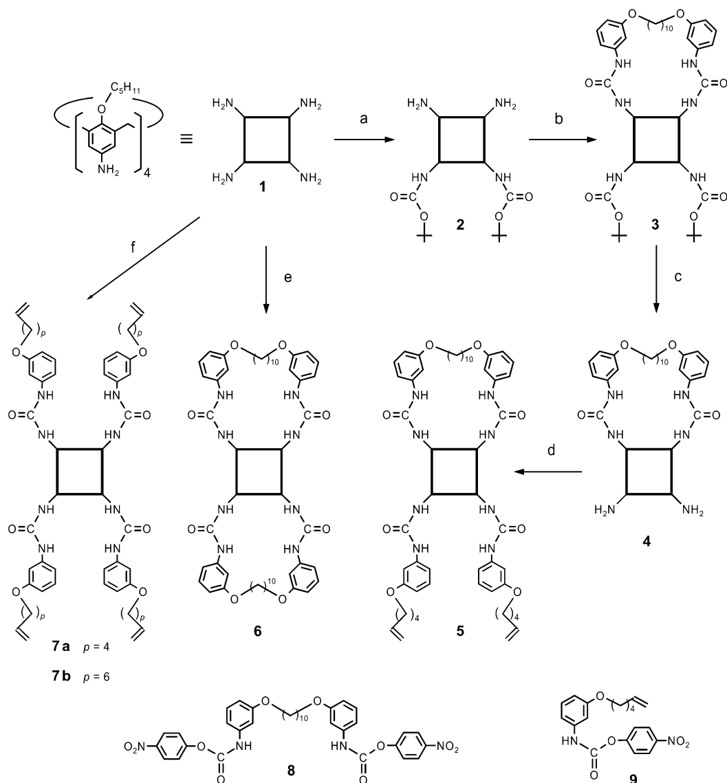
Scheme 1. Synthesis of mono-loop (5) and double-loop (6) tetraurea derivatives. The starting tetraaminocalix[4]arene tetraether in the cone conformation [30] is represented as a square (1). Conditions: a) see ref. [29]; b) DMF, Et 3 N, slow addition of 8 (1.25 mol), 74 %; c) TFA, CHCl 3 ; 4 h, 96 %; d) urethane 9 , CHCl 3 , 12 h, 96 %; e) similar to b (2.5 mol 8 ); f) urethane 9 , CHCl 3 , 12 h, 88 %.
