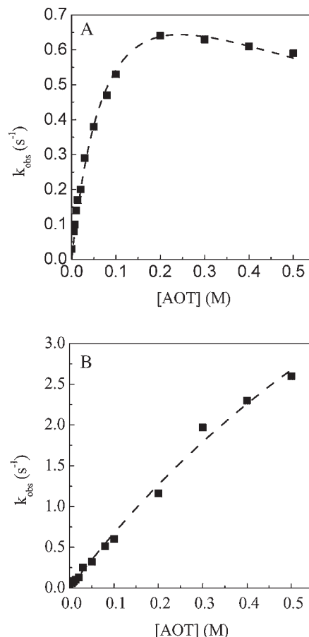
Figure 1. Dependence of k_{obs} with the AOT concentration, for the reaction between FDNB and PIP in: (A) EG/AOT/ n -heptane and (B) DMF/AOT/ n -heptane. [FDNB] = 1.0 \times 10^{-4} M, [PIP] = 0.015 M, W_s=2 . The dashed line shows the fitting by Eqn (11)
