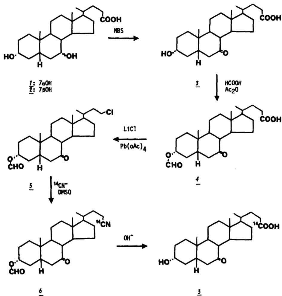
Figure 1: Preparation of ^{14}\text{C} -labeled cavicholic acid
