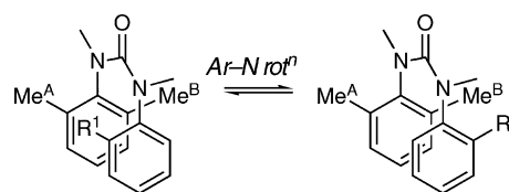
Fig. 1 Conformation and Ar–N rotation in 3l–u .
