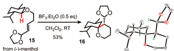
Figure 1. Cyclization of menthol-derived alkenyl acetal 15 . Molecular structure of product 16 as revealed by X-ray analysis. Selected hydrogen atoms have been added for clarity.
