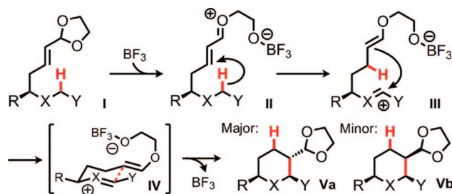
Scheme 2. Proposed Mechanistic Rationale
