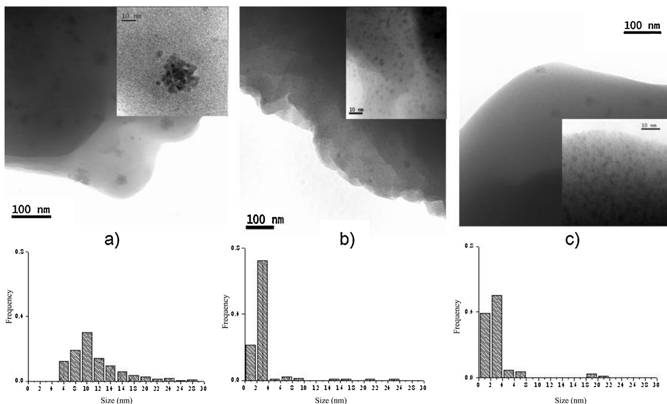
Fig. 2. Transmission electron micrographs and associated size distribution of matrix polymer embedded Pd nanoparticles: (a) pristine Pd-pol; (b) Pd-pol recovered after the first run of the reduction of quinoline with \text{NaBH}_4 ; (c) Pd-pol recovered after the seventh run of the reduction of quinoline with \text{NaBH}_4 .
