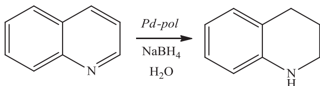
Scheme 2. Reduction of quinoline catalyzed by Pd-pol.
