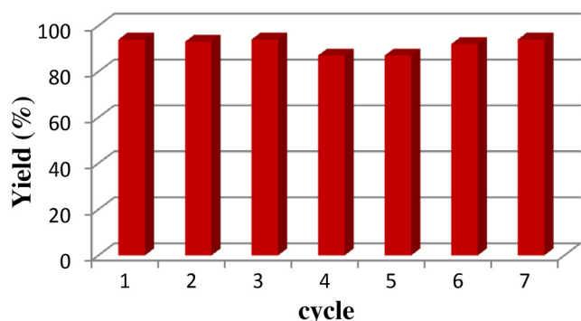
Fig. 1. Recyclability of Pd-pol (2.0 mol% of Pd) in the transfer hydrogenation of quinoline with NaBH 4 in water at 60 °C ( t = 9 h). Procedure A of the Section 2. GLC yields using biphenyl as the internal standard.
