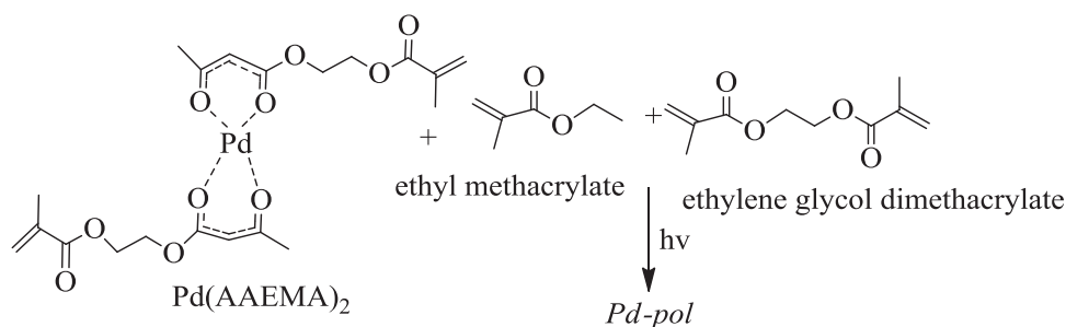
Scheme 1. Synthesis of Pd-pol.
