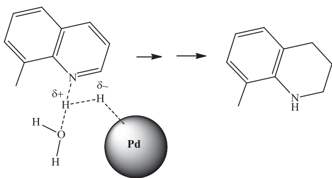
Scheme 5. Plausible transition state for the hydrogenation of 8-methylquinoline with Pd-pol in water.
