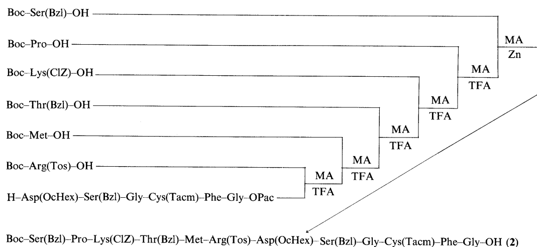
Fig. 5. Synthetic Scheme for the Protected Dodecapeptide Carboxylic Acid, Boc-(pBNP-32, 1-12)-OH (2)
