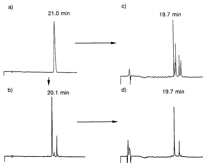
Fig. 3. HPLC Profile of Synthetic Somatostatin
