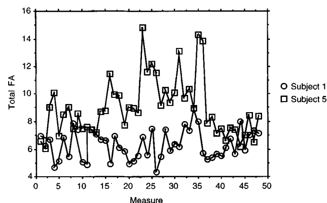
Figure 1 (Manning & Gage). Change in total FA in two subjects (1 and 5) with low and high F ratios, respectively. A similar pattern of change was obtained for relative FA scores.
