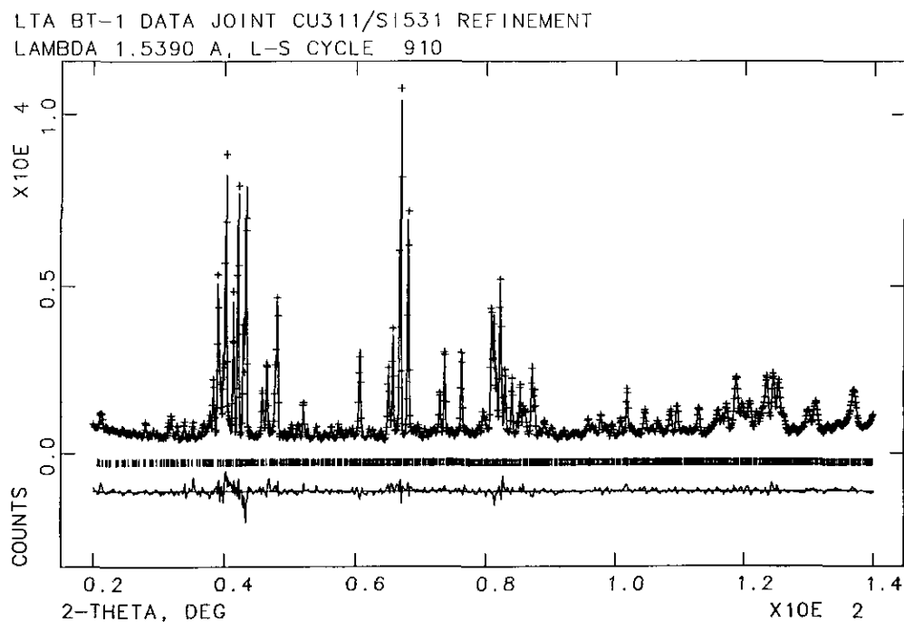
FIG. 2. Observed, calculated, and difference plots for the joint Rietveld refinement against neutron data (Cu(311) monochromator, \lambda = 1.539 \text{ \AA} ).
