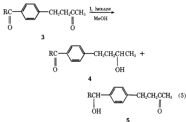
Isolated Yield of Ketol 4:5
