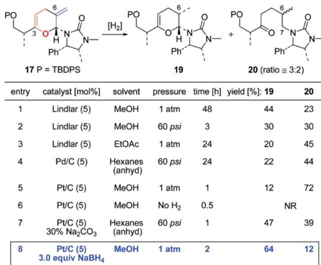
SCHEME 6. Hydrogenation of the C6 Exo-Cyclic Olefin in 17
