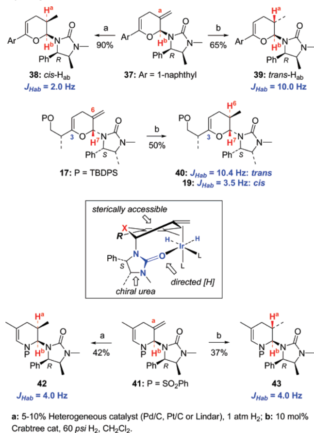
SCHEME 13. Scope of a Urea-Directed Stork–Crabtree Hydrogenation
