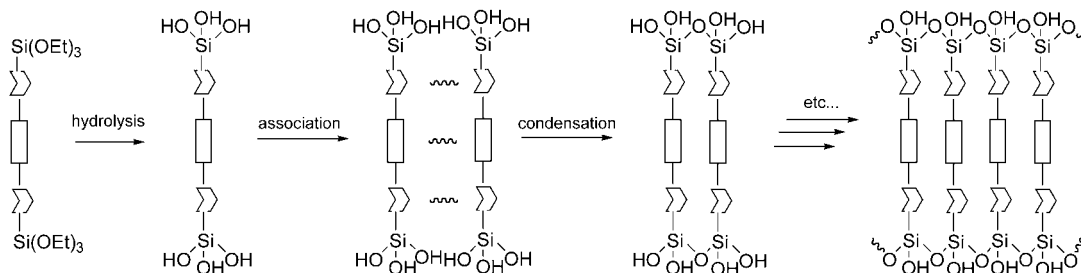
Scheme 5. Schematic representation of the hydrolysis–condensation process affording organised hybrids.
