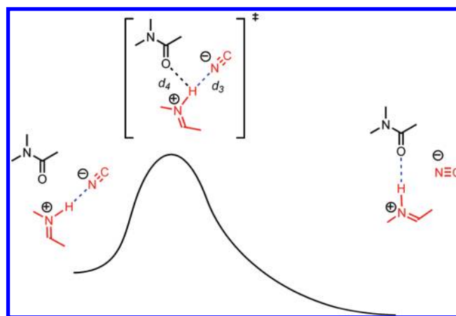
Figure 17. Qualitative reaction coordinate diagram for iminium/cyanide ion pair rearrangement depicting H-bond distances between iminium ion, cyanide anion, and catalyst amide.
