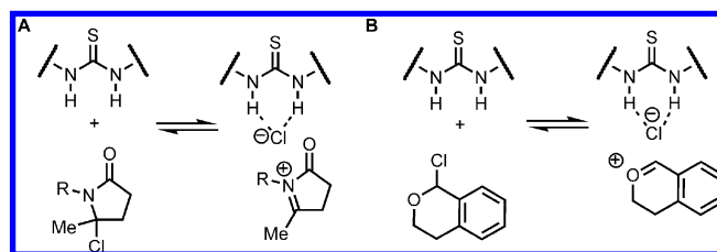
Scheme 2. Examples of Proposed Anion-Binding Mechanisms Promoted by Chiral (Thio)urea Derivatives Involving (A) N -acyl iminium/chloride and (B) Oxocarbenium/chloride Ion Pairs
