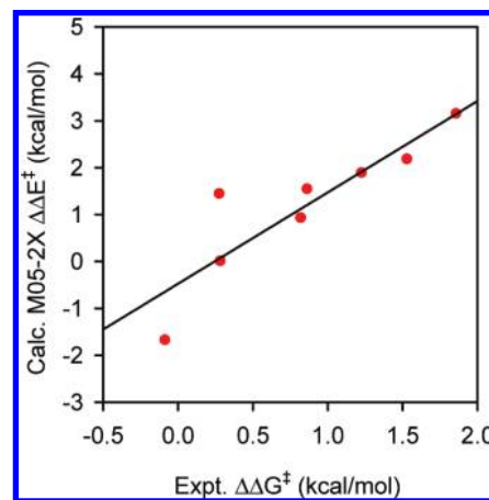
Figure 11. Calculated versus experimental enantioselectivity of HNC addition to 2a at the M05-2X/6-31+G(d,p)/B3LYP/6-31G(d) level. Plot of calculated \Delta\Delta E^\ddagger of HNC-addition transition structures versus estimated experimental \Delta\Delta G^\ddagger (Table 2, entries 1, 4–10). The curve represents a least-squares fit to f(x) = a + bx , a = -0.5 \pm 0.4 kcal/mol, b = 1.9 \pm 0.4 , R^2 = 0.79 , P_b = 0.0033 .
