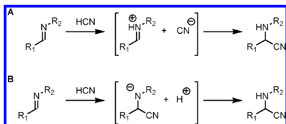
Scheme 5. Limiting Mechanisms for Imine Hydrocyanation Proceeding through (A) an Iminium Ion or (B) an \alpha -Aminonitrile Anion
