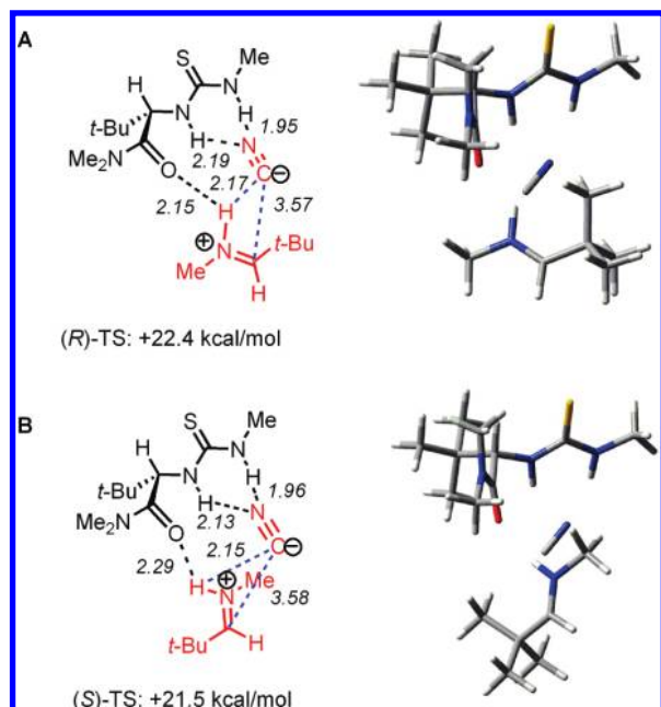
Figure 7. Calculated transition structures for HCN addition to imine 9a catalyzed by 8a (B3LYP/6-31G(d)). Transition structures leading to (A) ( R )- \alpha -aminonitrile and (B) ( S )- \alpha -aminonitrile are shown.
