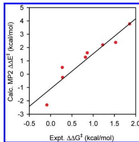
Figure 12. Calculated versus experimental enantioselectivity of HNC addition to 2a at the MP2/6-31G(d)/B3LYP/6-31G(d) level. Plot of calculated \Delta\Delta E^\ddagger of HNC-addition transition structures versus estimated experimental \Delta\Delta G^\ddagger (Table 2, entries 1, 4–10). The curve represents a least-squares fit to f(x) = a + bx , a = -1.1 \pm 0.4 kcal/mol, b = 2.6 \pm 0.4 , R^2 = 0.91 , P_b = 0.0003 .
