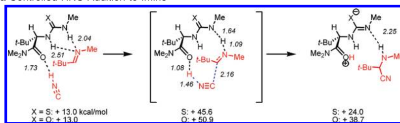
Scheme 6. Amido-(thio)urea Controlled HNC Addition to Imine a
