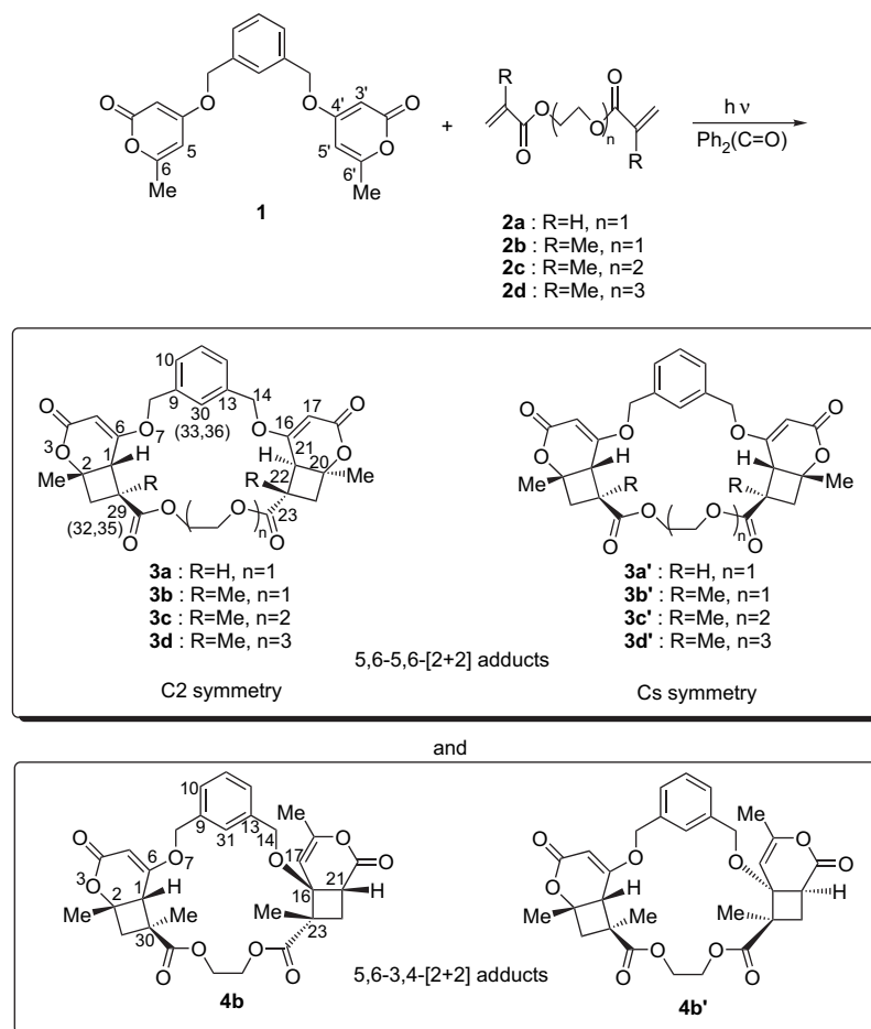
Scheme 1.
