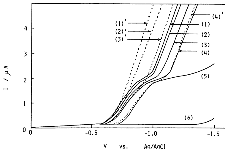
Fig. 1. Cathodic voltammograms of CySSCy in a Britton-Robinson buffer solution (pH 7.0) on various metal-fixed GCE 1 's (solid curves) and on bare metal wire electrodes (broken curves) at 2 mV s -1 in N 2 atmosphere.
