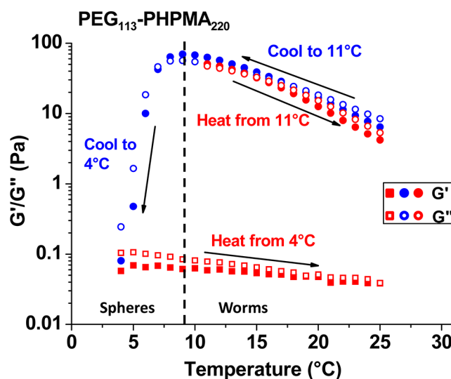
Figure 8. Storage ( G' ) and loss ( G'' ) moduli recorded for a 10% w/w PEG 113 -PHPMA 220 worm gel undergoing a temperature cycle between 25 and 4 °C (measurements were conducted at 1.0% strain and an angular frequency of 1.0 rad s -1 ).
