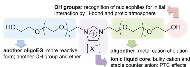
Figure 1. Concept of tailor-made ionic liquids: oligoether substituted imidazolium salts.
