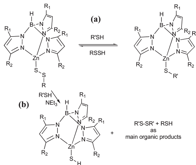
Scheme 2. Reaction of the Alkyldisulfanido Complexes with Thiols under Neutral and Basic Conditions
