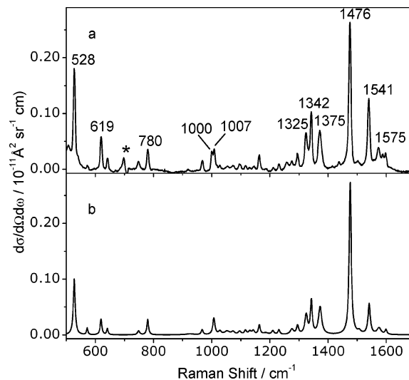
Figure 5. (a) Experimental resonance Raman spectrum for \text{Cu}(\text{pqx})(\text{PH}_3)_2^+ in dichloromethane solution. (b) Simulated spectrum. The dichloromethane solvents bands have been subtracted in the experimental spectrum. The asterisk indicates the residual from the subtraction process. The scale of the y-axis has been set by requiring the integrated band intensities to correspond to the values in the Supporting Information.
