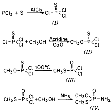
Figure 1 Scheme for the Synthesis of O,S-Dimethyl Phosphoroamidothioate
