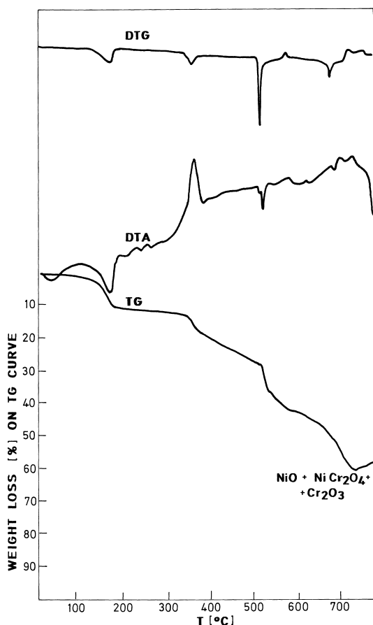
Fig. 4. TG, DTG and DTA traces for [\text{Nibpy}(\text{H}_2\text{O})_4]\text{CrO}_4 [A] in inert atmosphere.
