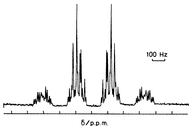
Figure. Proton-coupled ^{31}\text{P} n.m.r. resonances for \text{P}' in [\text{Ir}(\text{CO})-(\text{PEt}_3)_2(\text{P}'\text{H}_3)_2]^+ in \text{CD}_2\text{Cl}_2 at 190 K, recorded at 81 MHz
