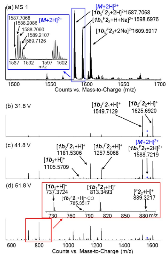
Figure 12. (a) Targeted doubly charged ion in MS1 stage for LC-MS/MS analyses. LC-QTOF (CID MS/MS) spectra of the isolated ^{\text{F}}\text{4b} at a collision energy of (b) 31.8, (c) 41.8, and (d) 51.8 V. The y-axis is normalized.
