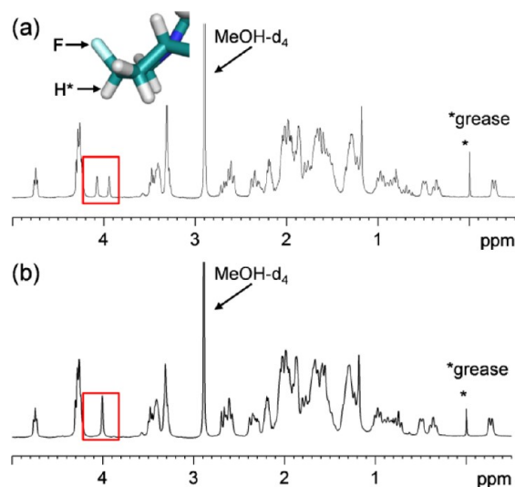
Figure 7. Portion ( \delta = -0.5 to 5.0 ppm) of 400.0 MHz ^1\text{H} NMR spectra of \text{F}^3\text{b} at 20^\circ\text{C} in 7\% \text{MeOH-}d_4/\text{CDCl}_3 : (a) ^{19}\text{F} coupled and (b) ^{19}\text{F} decoupled.
