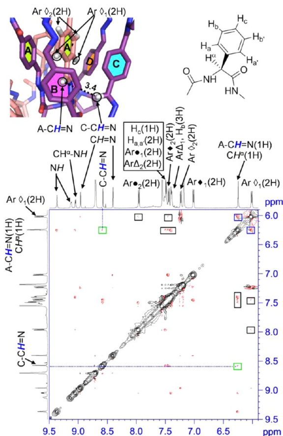
Figure 9. Portion of the 2D 500.1 MHz ROESY spectrum of F3d^{Ph} (F1 \delta = 5.9\text{--}9.5 ppm; F2 \delta = 5.9\text{--}9.5 ppm; pyridine- d_5 , 20 °C). Ar\blacklozenge_{1,2} , Ar\bullet_{1,2} , and Ar\Delta_{1,2} represent the remaining aryl ring CH's (B, C, and D). Inset: solid-state structure indicating Ar\blacklozenge_{1,2} neighboring imine CH groups in the ring A' and C (A-CH=N, and C-CH=N).
