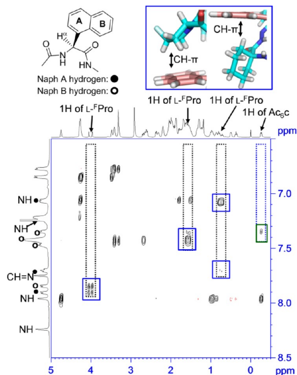
Figure 8. Portion of the 2\text{D } 600.1 MHz ROESY spectrum of \text{F}^3\text{b} ( \text{F1 } \delta = -0.5 to 5.0 ppm; \text{F2 } \delta = 6.5 – 8.5 ppm; 7\% \text{MeOH-}d_4/\text{CDCl}_3 , 20^\circ\text{C} ). Inset: solid-state structure showing CH- \pi interactions of a L-proline residue and an \text{Ac}_6\text{c} group to the naphthyl group.
