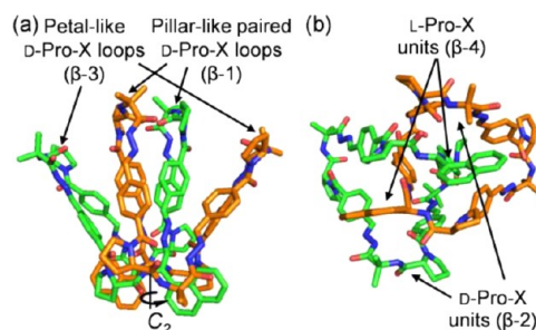
Figure 3. (a) X-ray structure of H 3 a displaying two identical interlocked tetramers. (b) View from the bottom of (a) along the C 2 axis showing a dense core. All hydrogen atoms are omitted for clarity.
