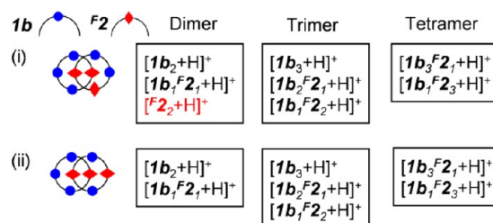
Scheme 2. Possible Daughter Ions for the Isomers of ^{\text{F}}\text{4b}
