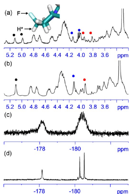
Figure 15. Portion ( \delta = 3.2 –5.3 ppm) of the 400.0 MHz ^1H NMR spectra of F4b at 20 °C in 7% MeOH- d_4 /CDCl _3 (a) coupled with ^{19}F and (b) decoupled with ^{19}F . The filled circles (red, blue, and black) indicate the H* signals of three L-FPro residues described in the insert picture. A portion ( \delta = -176 to -183 ppm) of the 400.0 MHz ^{19}F NMR spectra of F4b at 20 °C in 7% MeOH- d_4 /CDCl _3 , (c) ^1H coupled and (d) ^1H decoupled.
