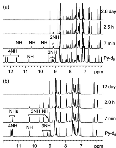
Figure 11. (a) Portion ( \delta = 5.8\text{--}12.5 ppm) of the 500.1 MHz ^1\text{H} NMR spectra of ^{\text{H}}\text{3c} (pyridine- d_5 (0.6 mL) + \text{D}_2\text{O} (0.03 mL), 20^\circ\text{C} ), recorded at different time from mixing. The bottom spectrum is the same portion of ^{\text{H}}\text{3c} in pyridine- d_5 before adding \text{D}_2\text{O} . (b) Portion ( \delta = 5.6\text{--}12.0 ppm) of the 500.1 MHz ^1\text{H} NMR spectra of ^{\text{F}}\text{3d}^{\text{Ph}} (pyridine- d_5 (0.6 mL) + \text{D}_2\text{O} (0.03 mL), 20^\circ\text{C} ), recorded at different time from mixing. The bottom spectrum is the same portion of ^{\text{F}}\text{3d}^{\text{Ph}} in pyridine- d_5 before adding \text{D}_2\text{O} .
