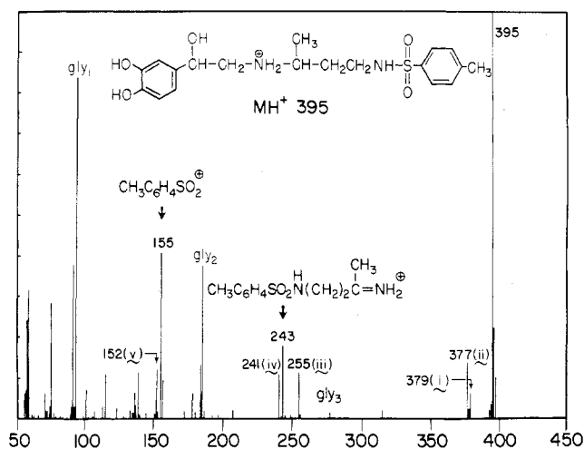
Figure 1. LSI mass spectrum of compound 25.
