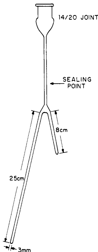
Figure 1. Sketch of the two-arm quartz ESR tubes.
