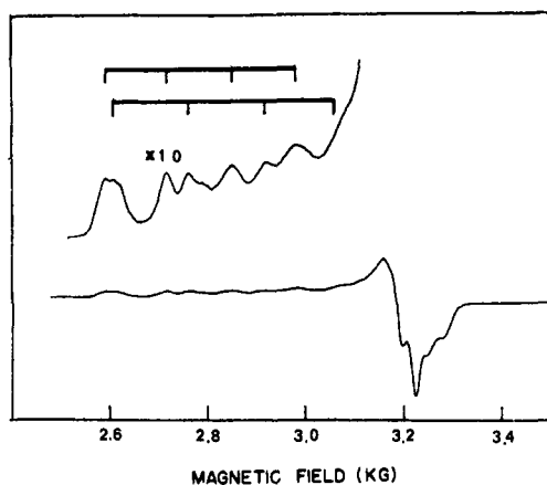
Figure 6. ESR spectrum of (e) in Figure 5 at higher gain. The conditions of the instrument are the same as for Figure 5 except a sweep rate of 125 G/min was used.
