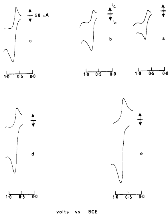
Figure 3. Effect of scan rate on the ratio of the peak currents (measured from the zero-current base-line level) of the anodic ( i_{\text{pa}} ) and cathodic ( i_{\text{pc}} ) cyclic voltammetric waves of (\text{TPP})\text{FeF}_2^- : dichloromethane solvent, 0.10 M \text{Pr}_4\text{NClO}_4 , 2.5 mM \text{Bu}_4\text{NF}\cdot 3\text{H}_2\text{O} , 1.0 mM (\text{TPP})\text{FeF} . Potentials are adjusted to the SCE reference: (a) 50 mV/s, i_{\text{pa}}/i_{\text{pc}} = 8.3 ; (b) 100 mV/s, i_{\text{pa}}/i_{\text{pc}} = 7.0 ; (c) 200 mV/s, i_{\text{pa}}/i_{\text{pc}} = 5.2 ; (d) 500 mV/s, i_{\text{pa}}/i_{\text{pc}} = 3.6 ; (e) 1 V/s, i_{\text{pa}}/i_{\text{pc}} = 2.9 .
