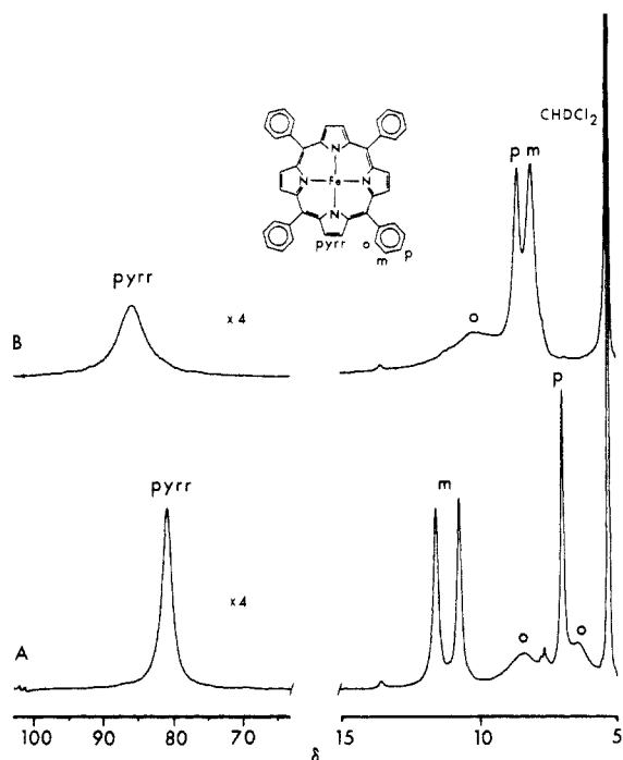
Figure 2. Downfield region of ^1\text{H} NMR spectra at 25 ^\circ\text{C} with \text{CD}_2\text{Cl}_2 as solvent and chemical shifts referenced to (\text{CH}_3)_4\text{Si} for (A) (\text{TPP})\text{FeF} and (B) (\text{TPP})\text{FeF}_2^- containing 10 mM \text{Bu}_4\text{NF}\cdot 3\text{H}_2\text{O} .
