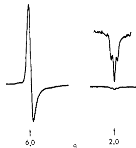
Figure 1. Electron spin resonance spectrum of ( p -OCH 3 TPP)FeF 2 - in 1/1 dichloromethane/toluene at -180 °C, 1 mM iron porphyrin, and 10 mM \text{Bu}_4\text{NF}\cdot 3\text{H}_2\text{O} .
