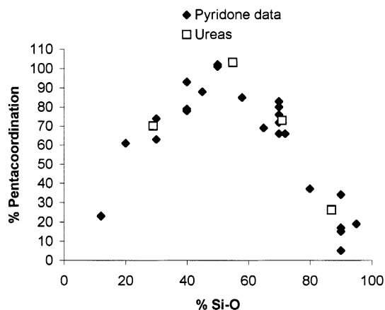
Fig. 2. Plot of % pentacoordination versus % Si–O bond formation.
